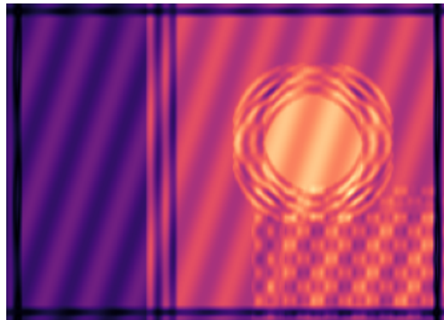
|Full - rank 4|, rel.err=0.00%
