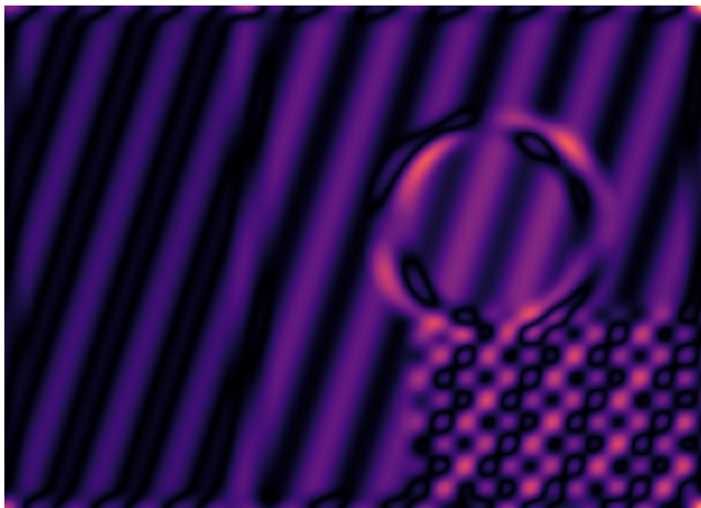
|Full - rank 1|, rel.err=1.15%
