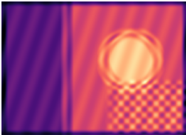
|Full - rank 2|, rel.err=0.88%
